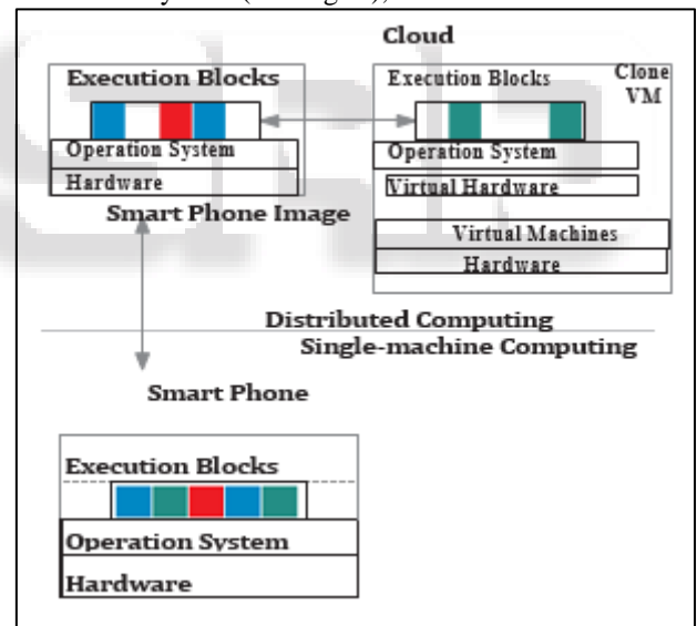
Fig. 4: Clone Cloud System Architecture
