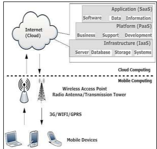
Fig. 3: Architecture of Mobile Cloud Computing
