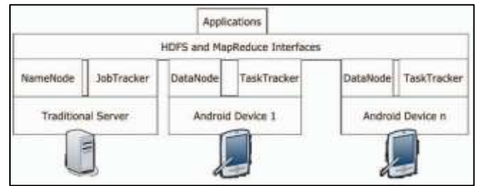
Fig. 7: Hyrax Infrastructure
