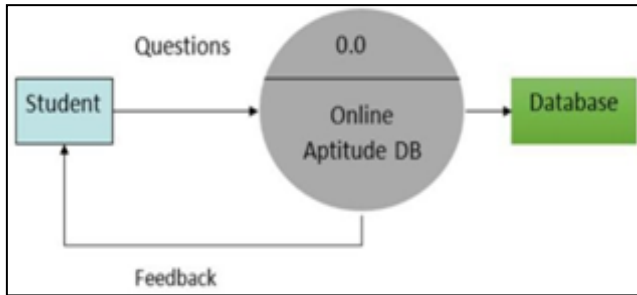
Fig. 2: DFD Level 0
