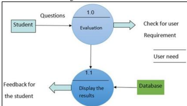
Fig. 3: DFD Level 1
