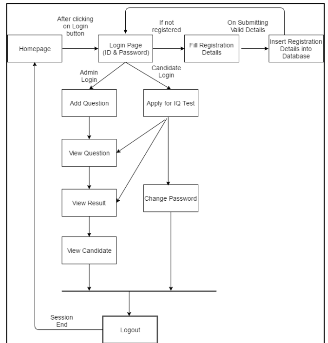
Fig. 1: Architecture
