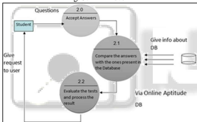
Fig. 4: DFD Level 2
