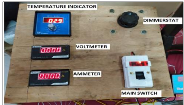
Fig. 2: Control Panel
