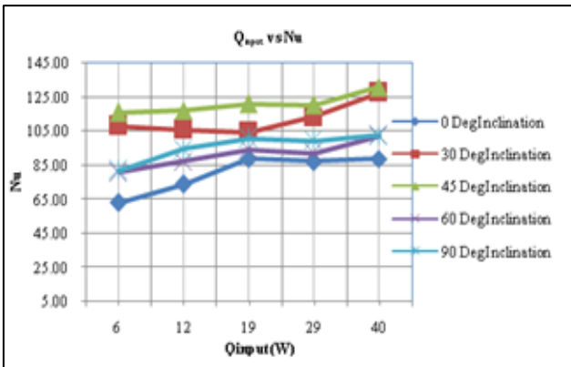
Fig. 4: x) Heat input Vs Nu for double row blind holes fin array
