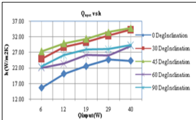
Fig. 4: vii) Heat input Vs Heat Transfer Coefficient for double row perforation fin array
