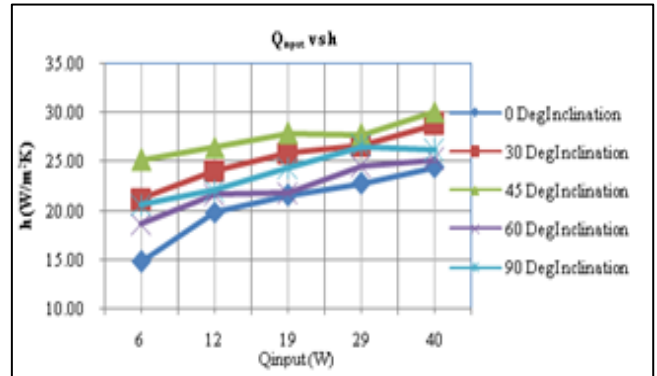
Fig. 4: v) Heat input vs Heat Transfer Coefficient for single row blind holes fin array
