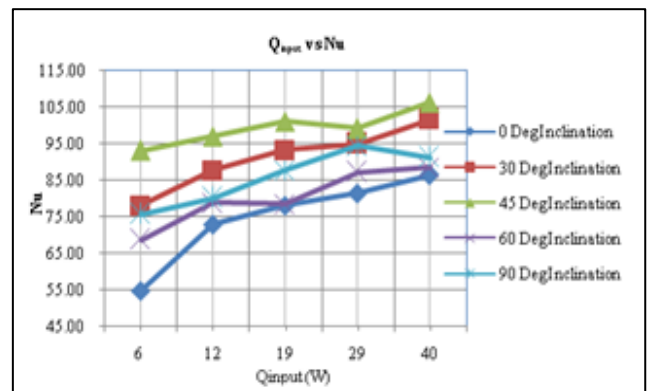
Fig. 4: vi) Heat input vs Nu for single row blind holes fin array
