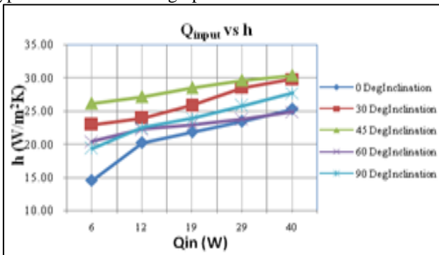
Fig. 4: i) Heat Input Vs Heat Transfer Coefficient for fin array without perforations
