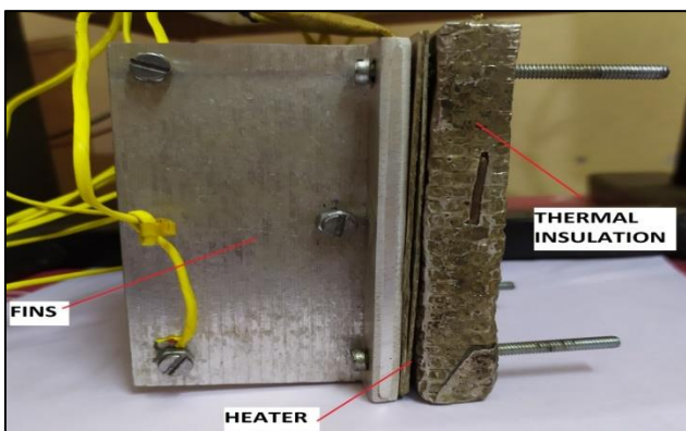
Fig. 1: Fin Array and Heater
