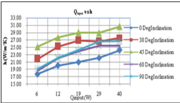
Fig. 4: iii) Heat input Vs Heat Transfer Coefficient for single row perforation fin array
