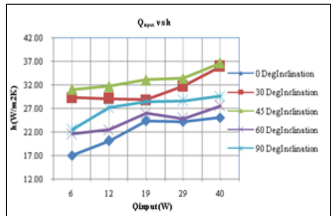
Fig. 4: ix) Heat input Vs Heat Transfer Coefficient for double row blind holes fin array
