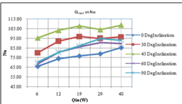
Fig. 4: iv) Heat input vs Nu for single row perforation fin array
