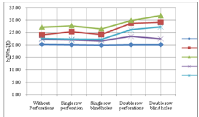
Fig. 4: xii) Effect of geometry and inclination on heat transfer coefficient at 12W heat input
