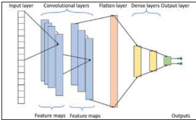
Fig. 8: CNN Architecture
