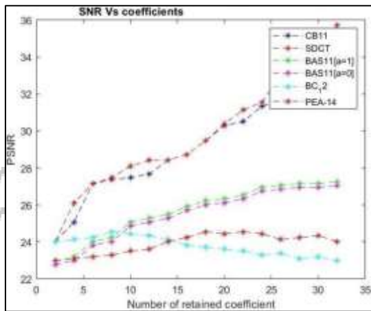
Fig. 5: Approximate DCT compression of an image using inexact adders PSNR vs Number of retained coefficient
