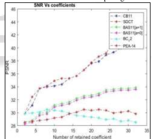
Fig. 2: Approximate DCT compression of an image using inexact adders PSNR vs Number of retained coefficient
