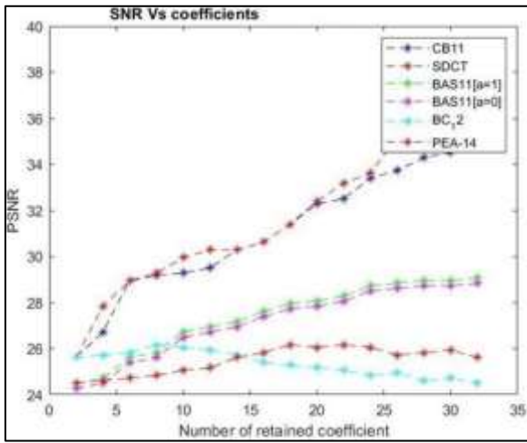
Fig. 4: Approximate DCT compression of an image using inexact adders PSNR vs Number of retained coefficient
