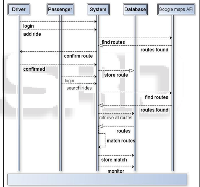
Fig. 1: Sequence Diagram-matching a shared ride for a driver and a passenger
