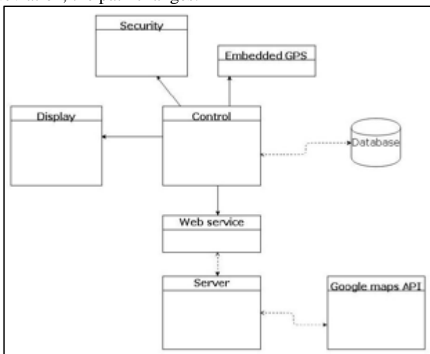
Fig. 4: Object Diagram
