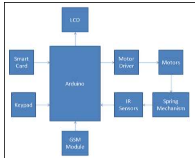
Fig. 1: Block Diagram
