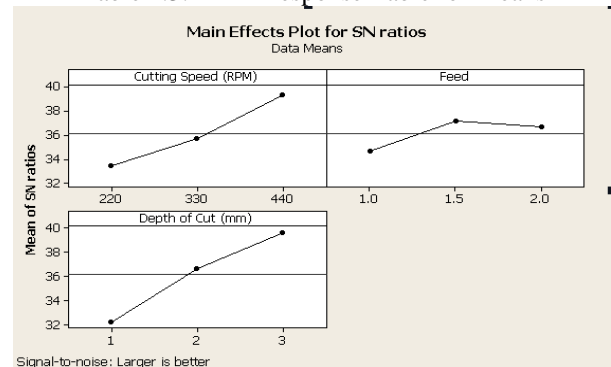
2.1 Main effects of Plot for S/N Ratio Material Removal Rate
