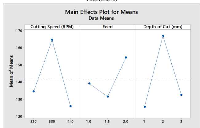
Graph 3.2 Main effects of Plot for Means of Hardness
