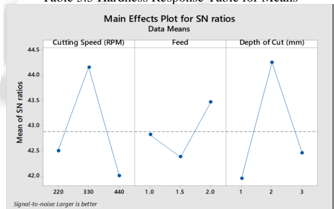
Graph 3.1 Main effects of Plot for Signal to noise Ratio of Hardness
