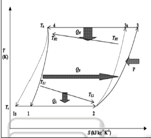
Fig. 1: Stirling Heat Pump cycle
