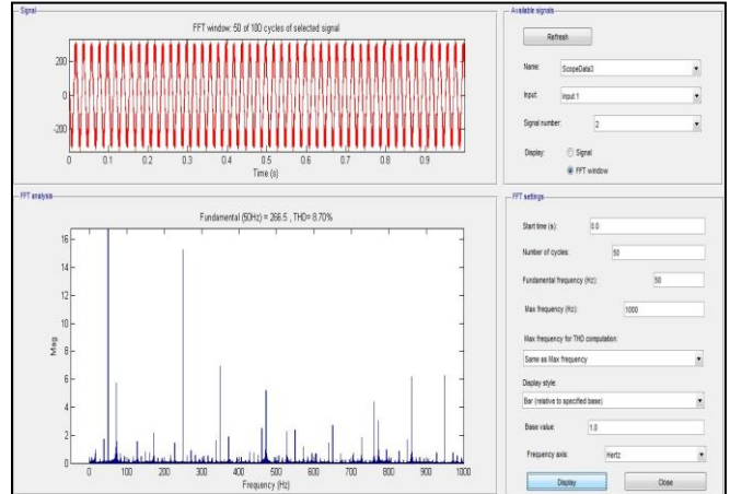
Fig. 7: FFT Analysis of Phase Voltage 7 Level NPC Inverter
