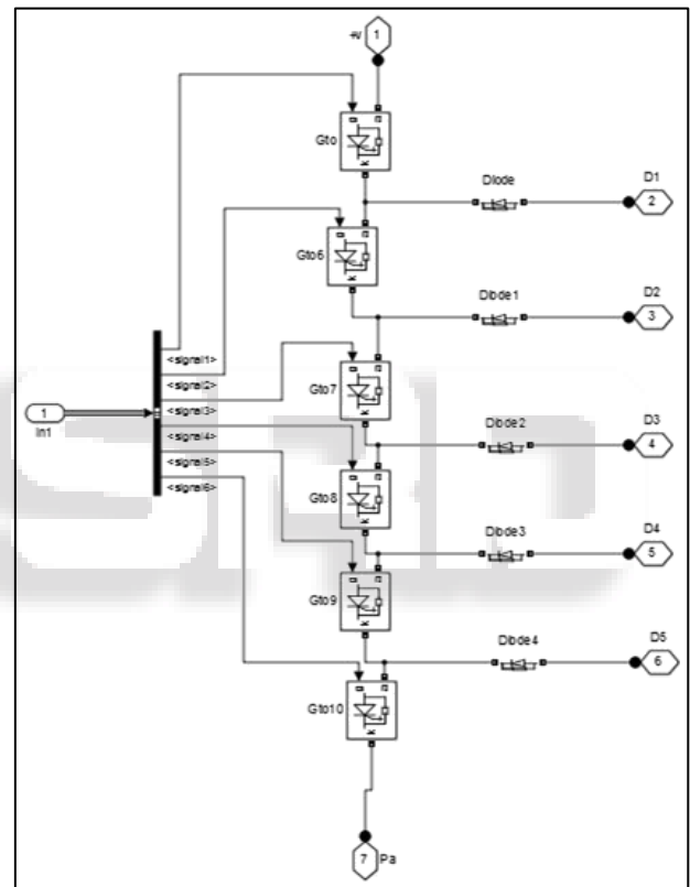
Fig. 3: Subsystem of Pulse Generation
