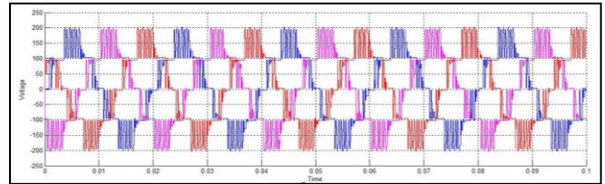
Fig. 6: Simulation Signal Analysis of 7 Level NPC Inverter
