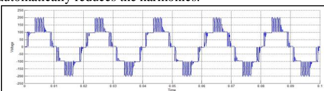
Fig. 5: Output of 7 Level NPC Multilevel Inverter
