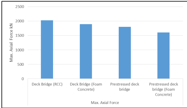
Fig. 4: Max. Axial force
