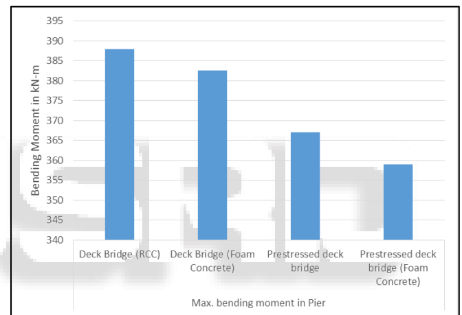
Fig. 2: Bending moment
