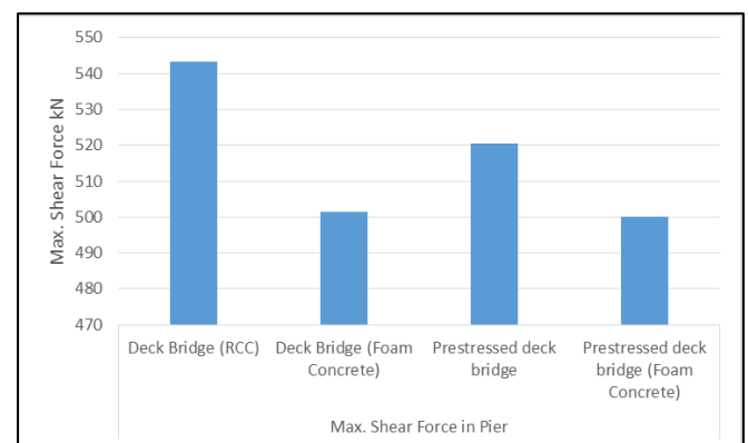
Fig. 3: Max. Shear Force
