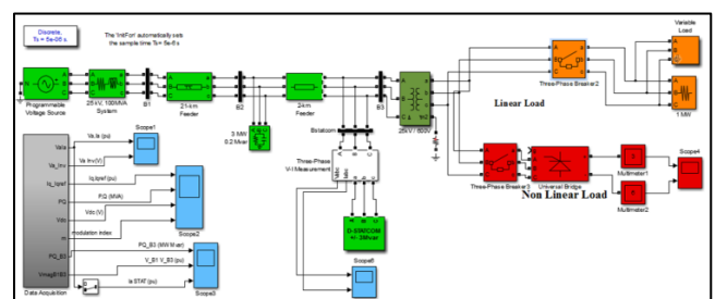
Fig. 2: MATLAB model of DSTATCOM circuit.
