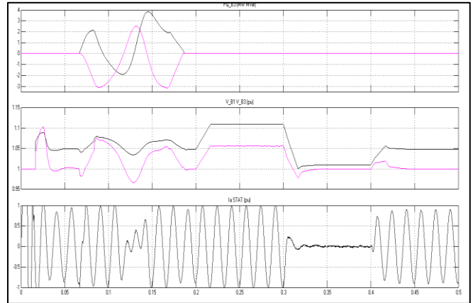
Fig. 7: Scope 3 Simulation Result
