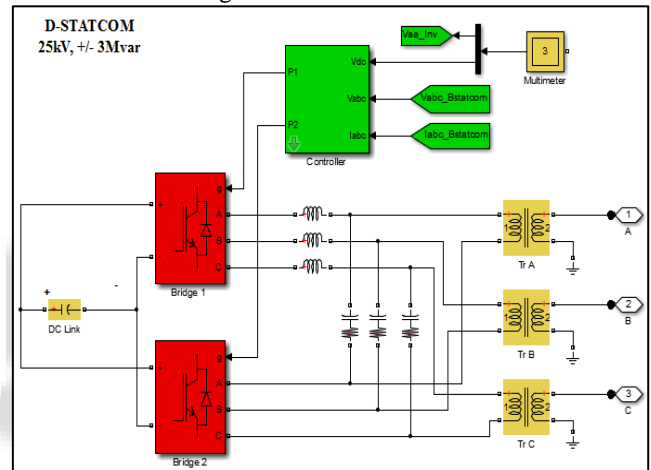
Fig. 2: MATLAB model of DSTATCOM circuit.
