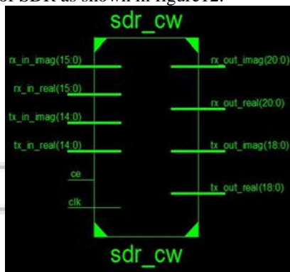
Fig. 11: RTL schematic of SDR
