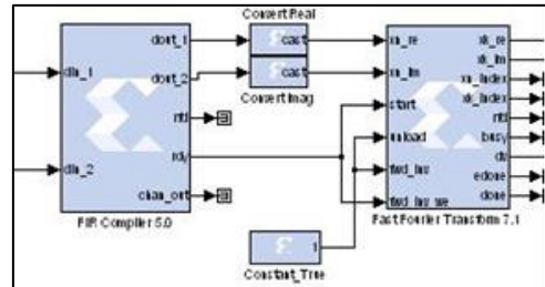
Fig. 5: Channelizer of SDR
