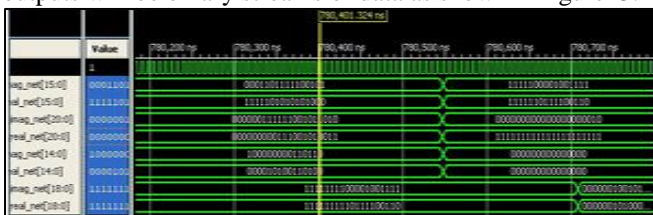
Fig. 13: SDR model waveform
