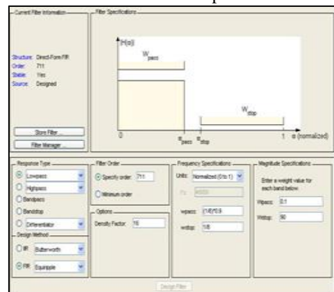
Fig. 7: Design of Filter in FDA Tool
