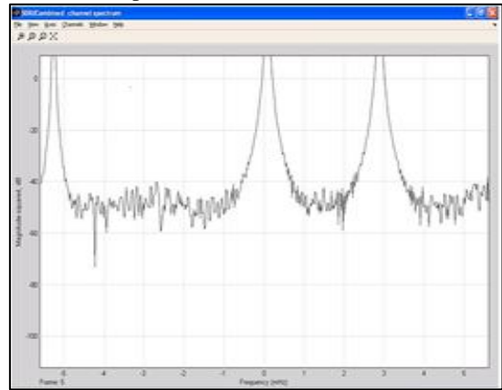
Fig. 14: SDR combined channel spectrum output
