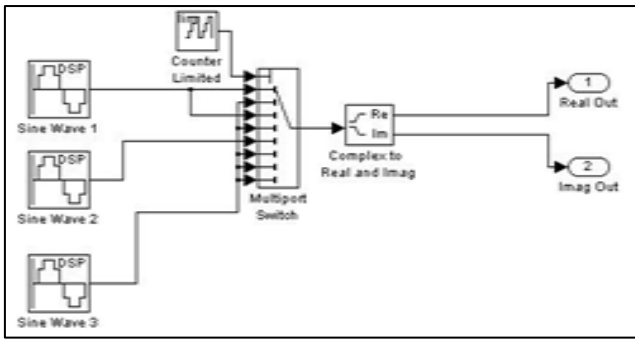
Fig. 2: channel sources for the SDR
