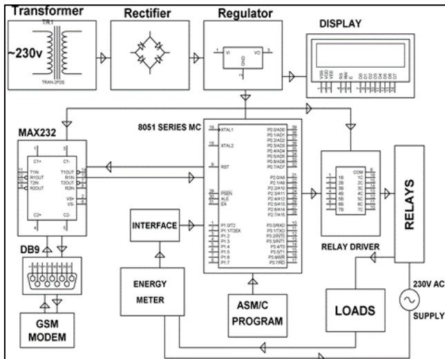
Fig. 1: Block diagram of power meter billing plus load control using GSM
