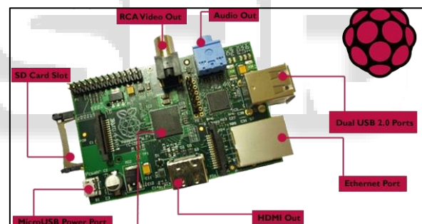
Fig. 1: Raspberry PI-3
