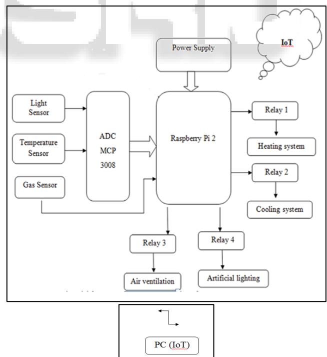
Fig. 1: Green House Energy System
