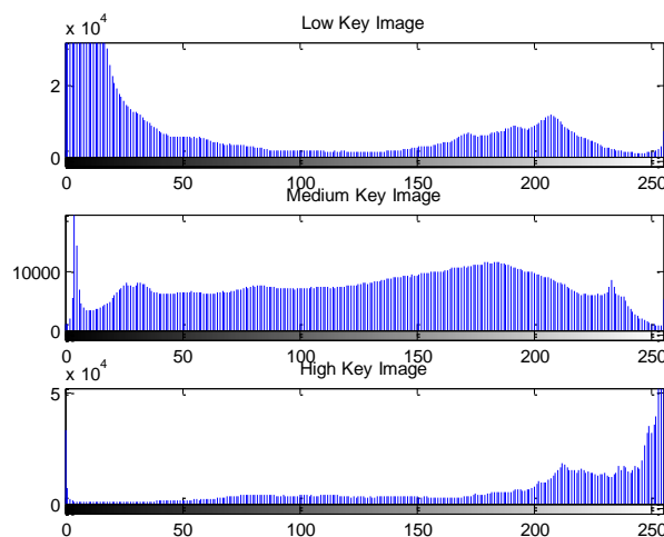
Fig. 6: Histograms of images
