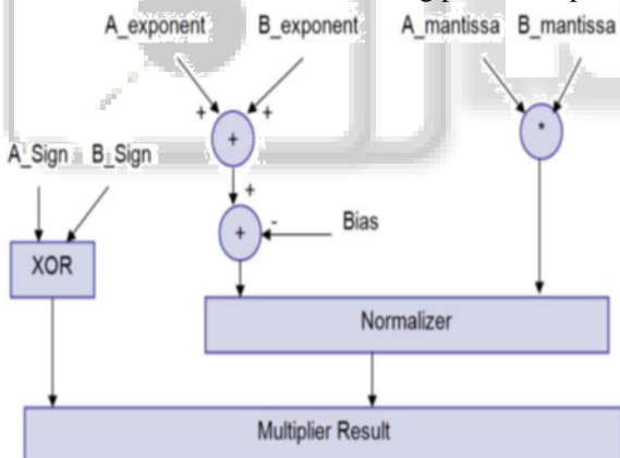
Fig. 2.1: Floating point multiplier block diagram
