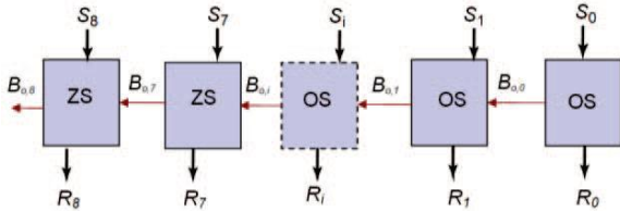
Fig. 2.4: Ripple Borrow Subtractor
