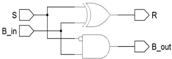
Fig. 2.3: bit subtractor with the input T = 0
