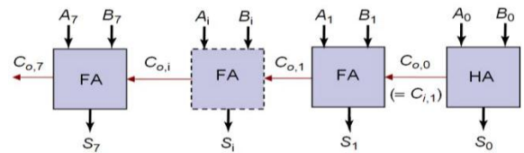
Fig. 2.2: Ripple Carry Adder
