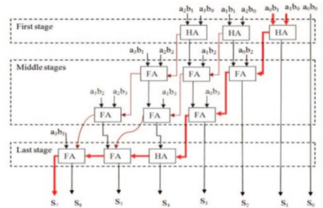
Fig. 2.5: 4x4 bit Carry Save multiplier
