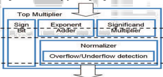
Fig. 3.1: Floating point multiplier with pipelined stages
