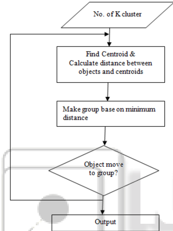
Fig. 2: Flowchart of K-mean clustering algorithm
