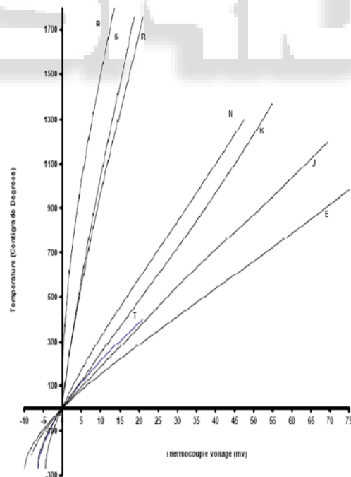
Fig. 4 Voltage-Temperature Characteristics of B, E, J, K, N, R, S, and T Type Thermocouples
