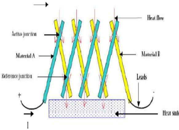
Fig. 5 Schematic of Thermopile
