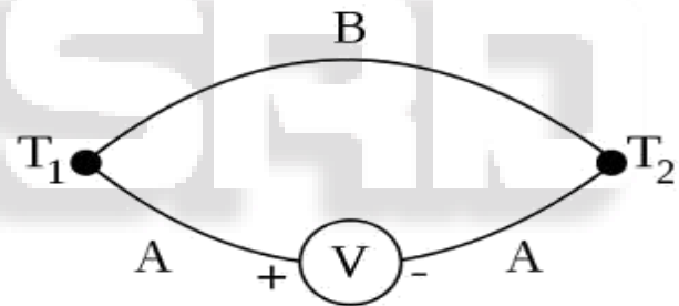
Fig. 1 Illustration of Seebeck Effect
