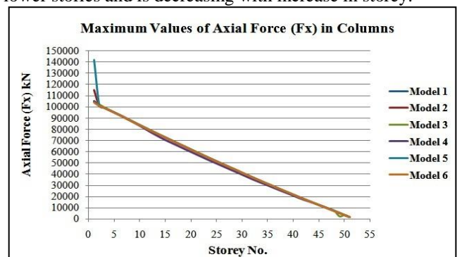
Fig. 1: Maximum Values of Axial Force ( F_x ) in Columns Considering Seismic Forces
