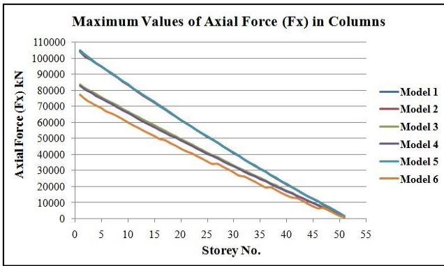
Fig. 2: Maximum Values of Axial Force ( F_x ) in Columns Considering Wind Forces
