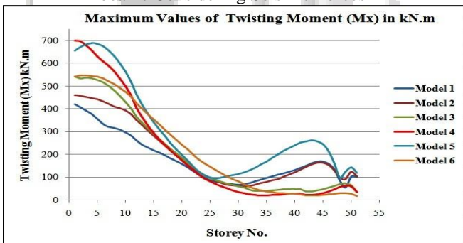
Fig. 4: Maximum values of Twisting Moment ( M_x ) in beams Considering Wind Forces
