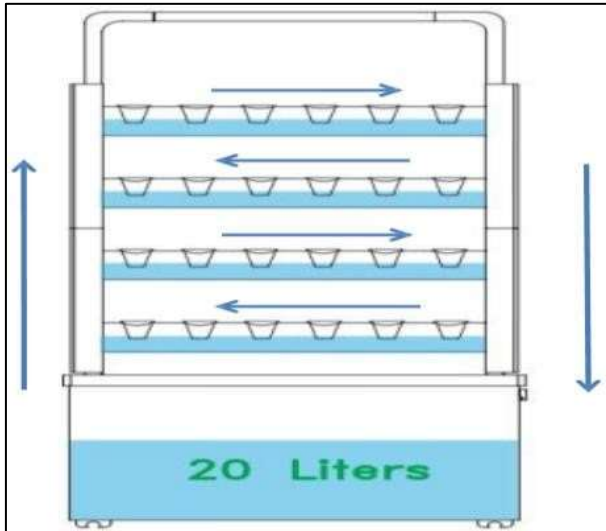
Fig. 12: Final Prototype.
