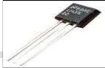
Fig. 6: LM35 Sensor
