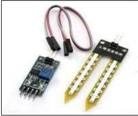
Fig. 8: Moisture Sensor
