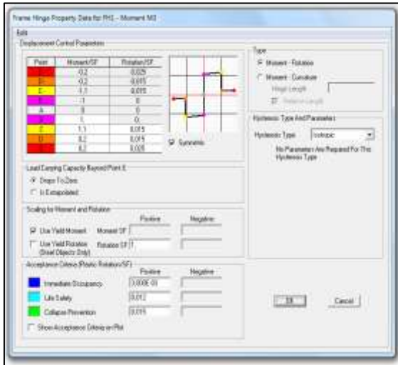
Fig. 3: Hinge Properties for Beam
