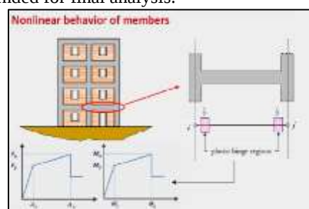
Fig. 1: Nonlinear behavior of member
