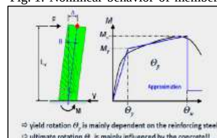
Fig. 2: Yield rotation for concrete & steel
